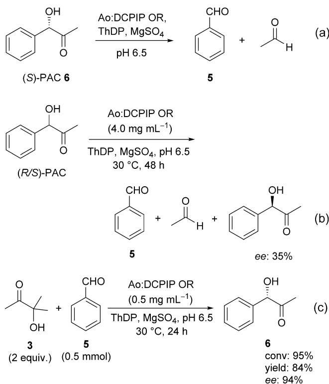
Scheme 3. Cleavage of ( S )- and ( rac )-PAC [Eq. (a) and (b)] and optimized conditions for the synthesis of ( S )-PAC ( 6 ).
