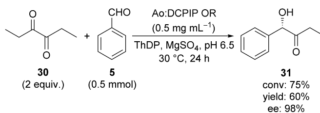
Scheme 4. Approaching the class of ( S )-phenylpropionyl carbinol derivatives (PPCs) by Ao:DCPIP OR catalysis.
