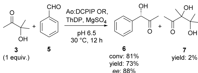
Scheme 2. Explorative study of the cross-benzoin-like reaction of methylacetoin ( 3 ) and benzaldehyde ( 5 ) catalyzed by Ao:DCPIP OR.
