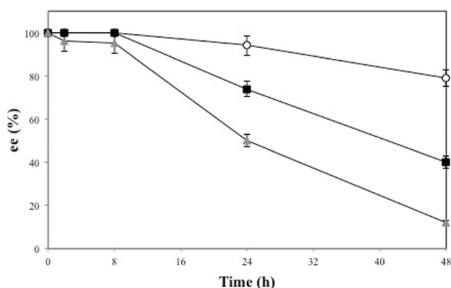
Figure 3. Enantiomeric excess of 6 as a function of time at different enzyme concentrations (○: 0.5 mg mL -1 ; ■: 2.0 mg mL -1 ; ▲: 4.0 mg mL -1 ). Values are the mean ±SD of triplicates.
