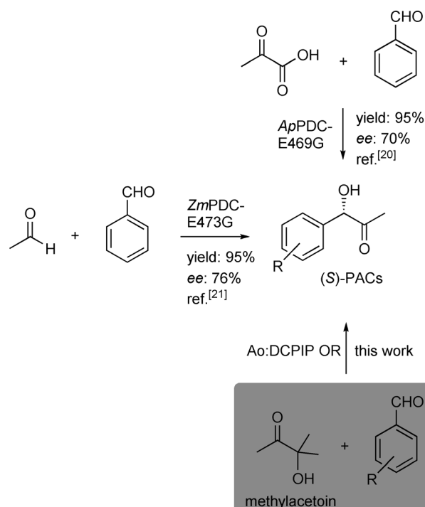
Figure 1. Enzymatic carboligations for the direct asymmetric synthesis of ( S )-phenylacetyl carbinols (PACs).
