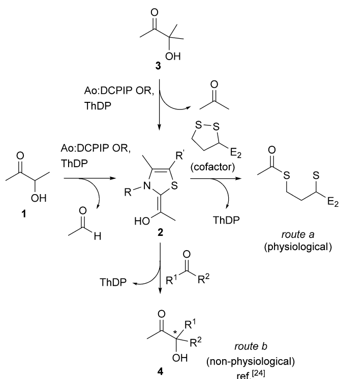
Scheme 1. Physiological and non-physiological activities of Ao:DCPIP OR. R = (4-amino-2-methylpyrimidin-5-yl)methyl; R' = ethyl diphosphate. Cofactor = lipoamide covalently bound to the second enzyme system (AoDH ES).
