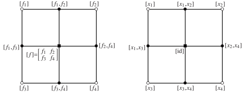
FIGURE 3. Generic big square &amp; standard big square.
