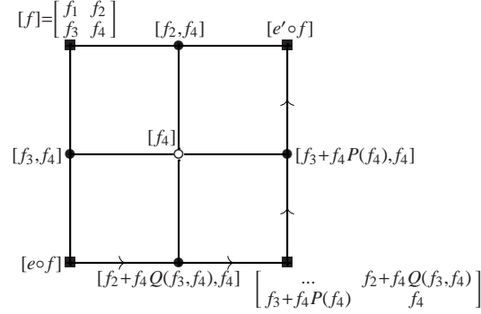
FIGURE 10. Local homotopy in Case (2): P \in \mathbb{C}[f_4] .
